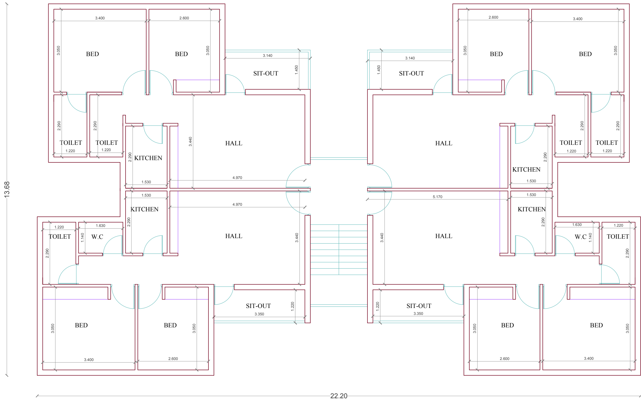
TYPICAL FLOOR PLAN
